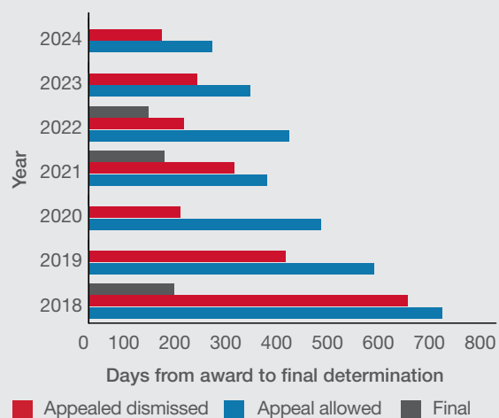
Graph 3: Average days from award to final determination
