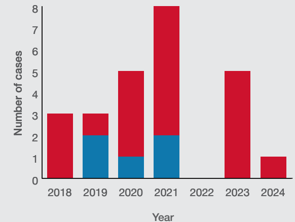
Graph 5: Success rate of the appealed High Court and SICC decisions from 2018 to 2024
