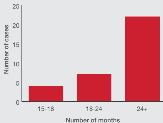
Graph 9: Number of reported appeal decisions from 2018 to 2024 measured against the time taken to issue award
