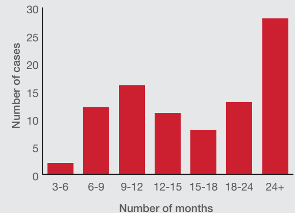
Graph 10: Number of reported final decisions from 2018 to 2024 measured against time taken to issue award
