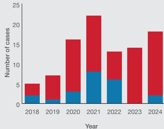
Graph 4: Success rate of all reported decisions from 2018 to 2024
