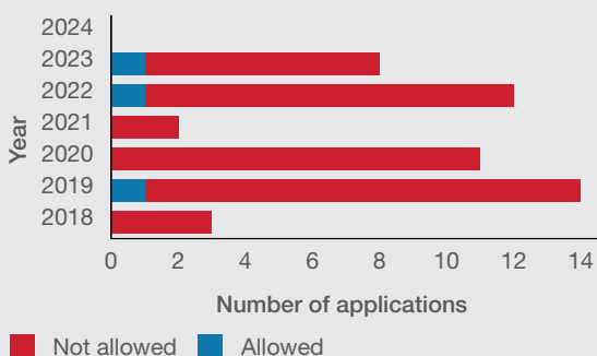
Graph 4: Art. 34(2)(a)(i) applications per year
