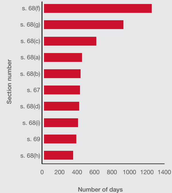
Graph 7: Average time for decision on challenge by ground
