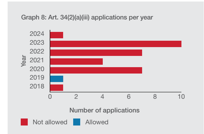
Graph Article 34(2)(a)(iii)
