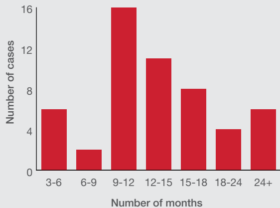
Graph 8: Number of reported first instance decisions from 2018 to 2024 measured against time taken to issue award
