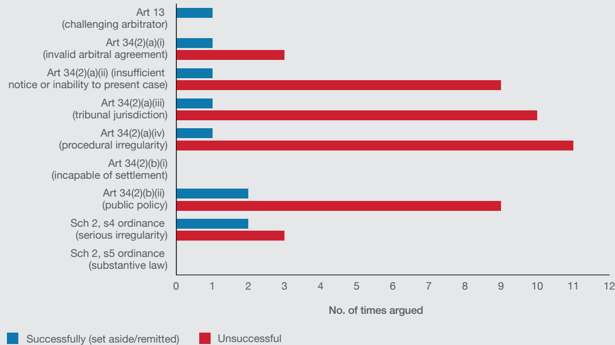
Graph 7: Distribution of grounds argued
