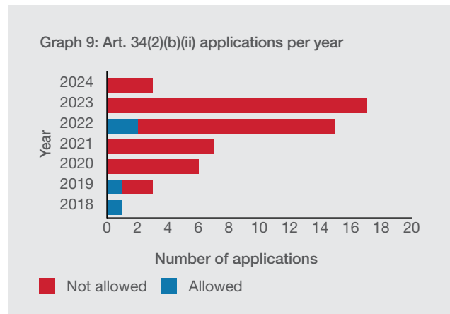
Graph Article 34(2)(b)(ii)
