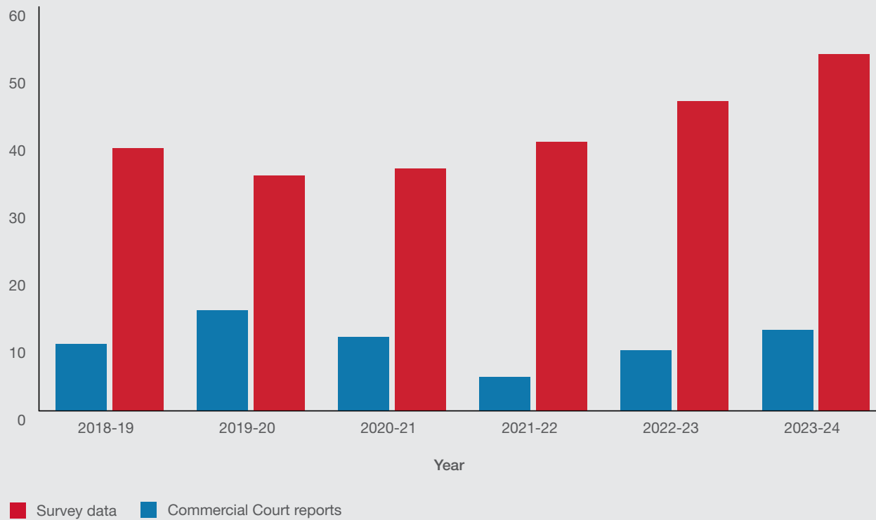
Graph 10: Number of Section 69 challenges in survey data vs. Commercial Court reports
